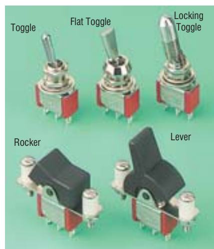
Toggle panel cut-out=6.35 dia
